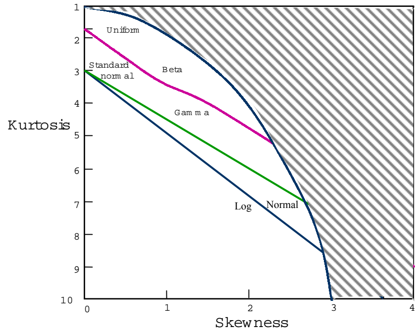
Skewness - Kurtosis Chart for the Major Distributions
