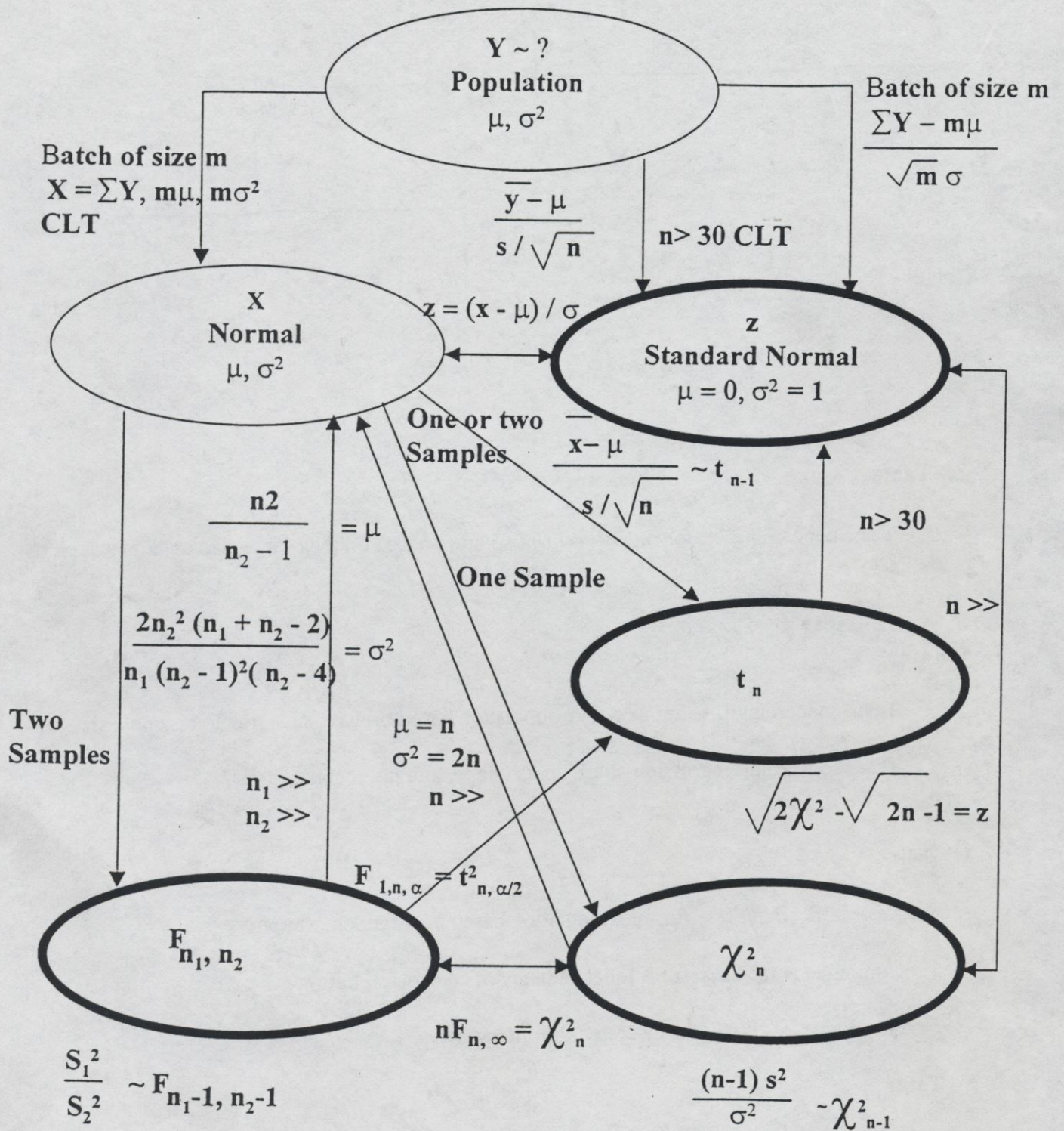
Relationship Among Statistical Tables and Their Applications
